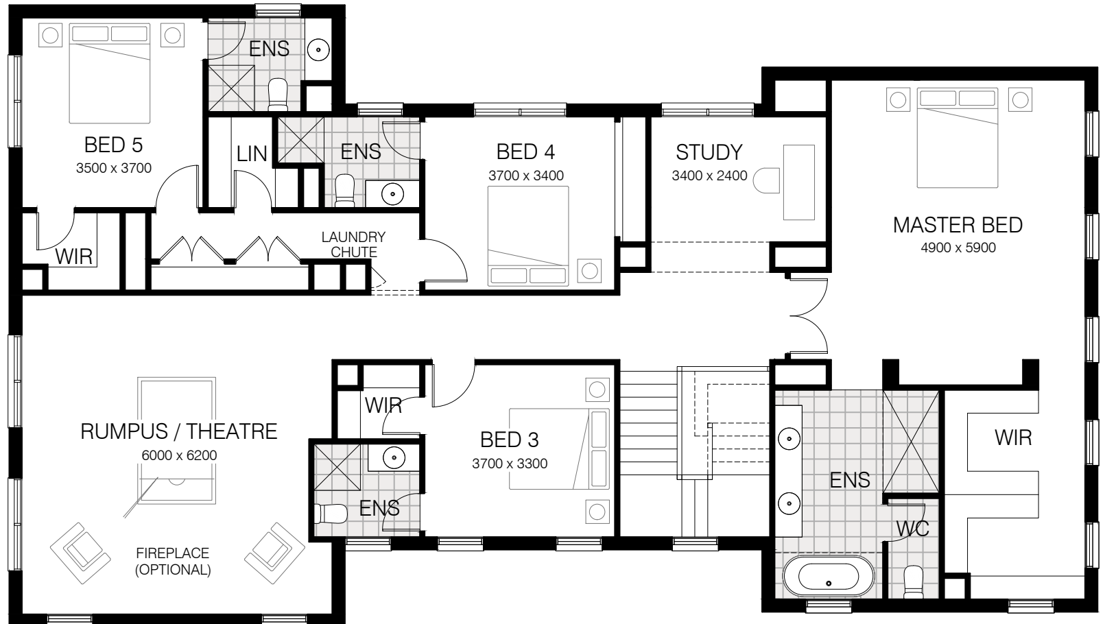
FIRST FLOOR
